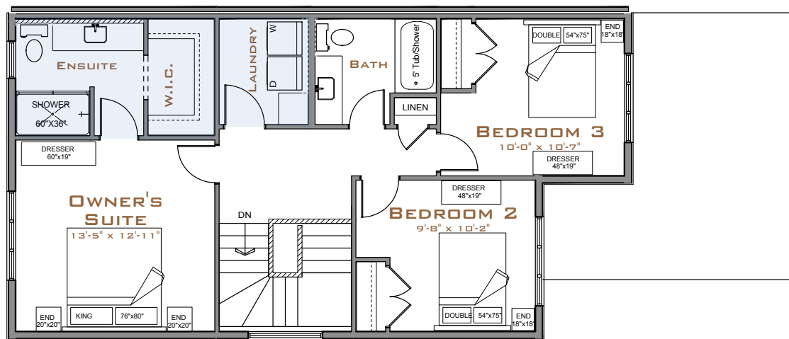
OPTION 2 - UPPER FLOOR – 861 SQ.FT. LARGER ENSUITE / LAUNDRY ROOM / WALK-IN-CLOSET
